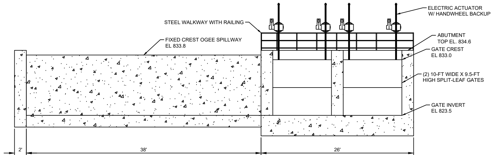
DOWNSTREAM ELEVATION VIEW
