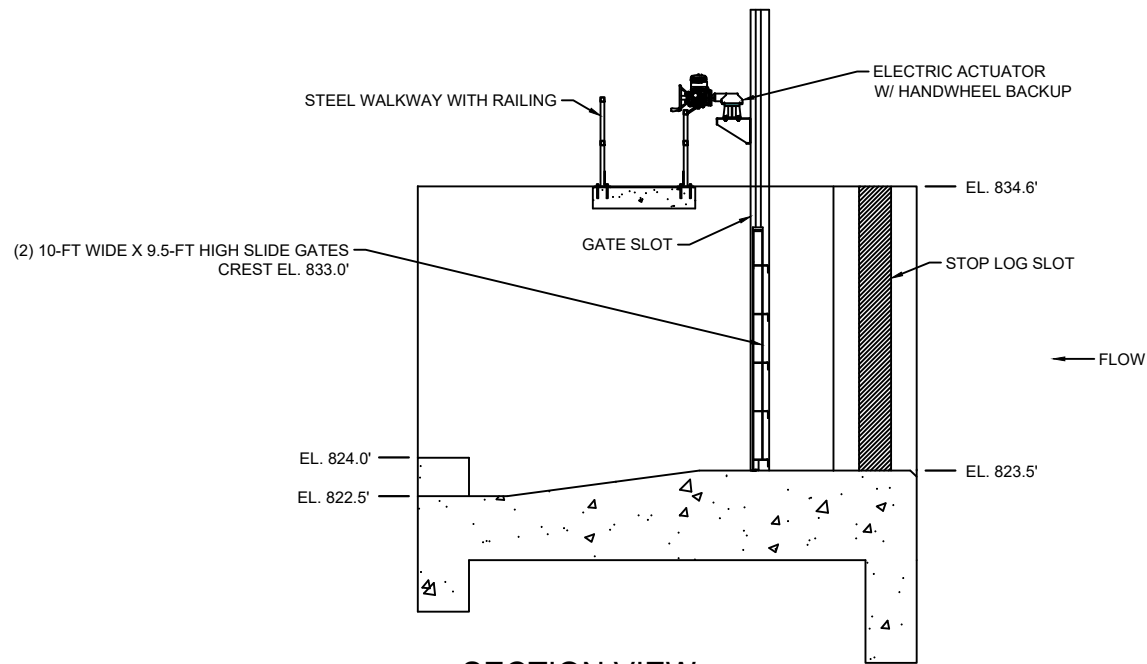
SECTION VIEW
