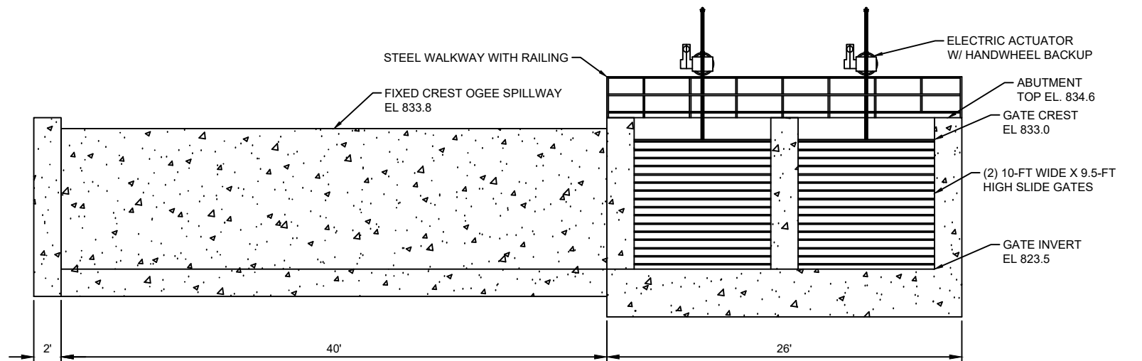
DOWNSTREAM ELEVATION VIEW
